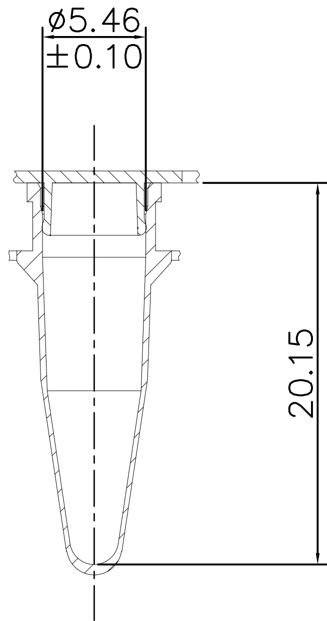
SECTION thro' TUBE & CAP 8pos
